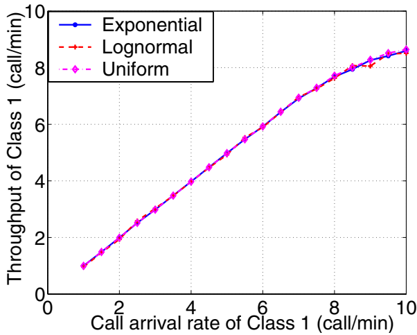
Fig. 9. Throughput of class 1 under different distributions of workload: Exponential distribution; Lognormal distribution; Uniform distribution. Dynamic p(t) \in [0.0234, 0.1667] .
