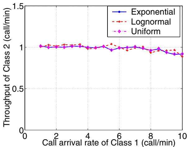
Fig. 10. Throughput of class 2 under different distributions of workload: Exponential distribution; Lognormal distribution; Uniform distribution with dynamic p(t) \in [0.0234, 0.1667] .
