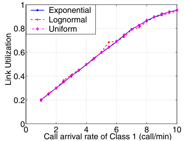
Fig. 11. Link utilization under different distributions of workload: Exponential distribution; Lognormal distribution; Uniform distribution with dynamic p(t) \in [0.0234, 0.1667] .
