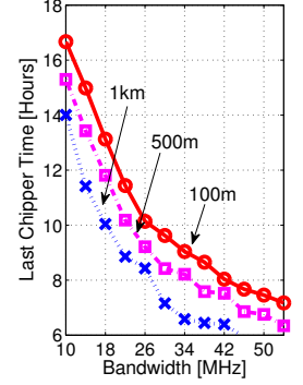
Fig. 13. Last chipper time with different mobility radii.
