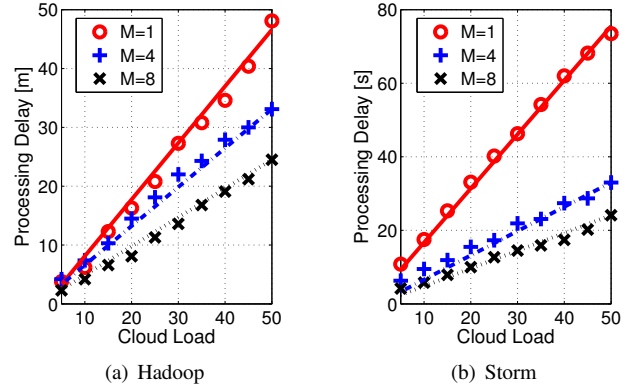
Fig. 10. The processing delay versus constant cloud load L in Hadoop and Storm with different numbers of computers M used in the cloud.
