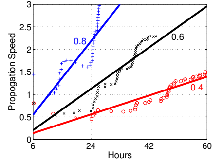
Fig. 6. Propagation speed over time for vulnerable ratio \kappa=0.4, 0.6, and 0.8 .
