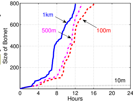
Fig. 8. Size of the botnet over time with mobility radius \alpha=10, 100\text{m}, 500\text{m} , and 1\text{km} .
