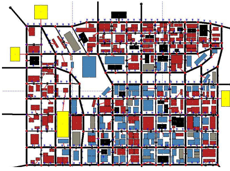
Fig. 7. 2km×2km map in downtown Chicago used in experiments (Courtesy of [22]).
