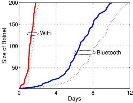
Fig. 4. Size of the botnet over time for two starting nodes: node “abmuyawm” – solid line, node “oafhynu” – dotted line.
